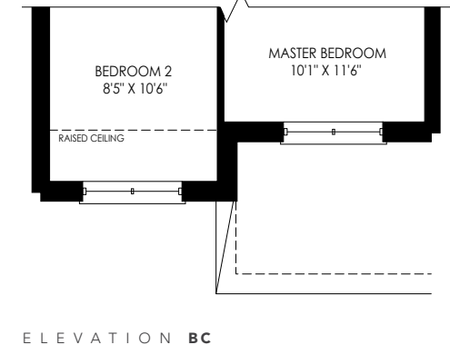
ELEVATION BC
