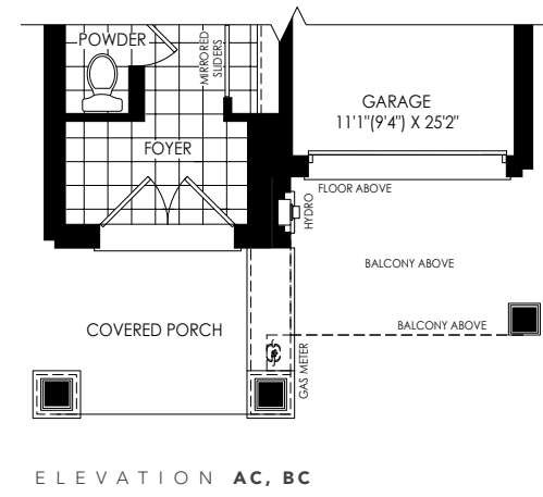
ELEVATION AC, BC
